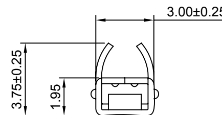
SEC:C-C
