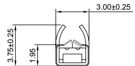
SEC:C-C
